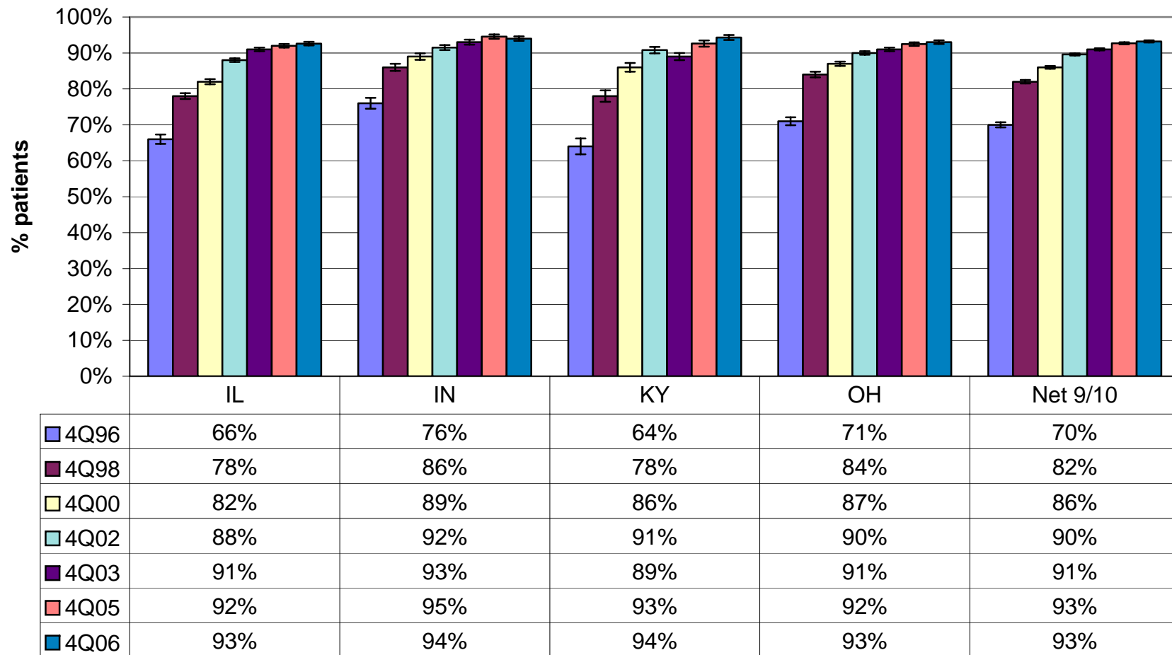
Percentage of HD Patients with Reported Kt/V \geq 1.2 by State and Network 9/10 for Selected Collection Periods
